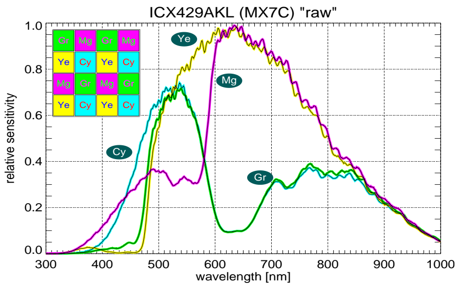
Fig. 5. Spectral response of four channel (CYGM) Sony ICX429AKL CCD in “raw” mode with color mosaic inset.
