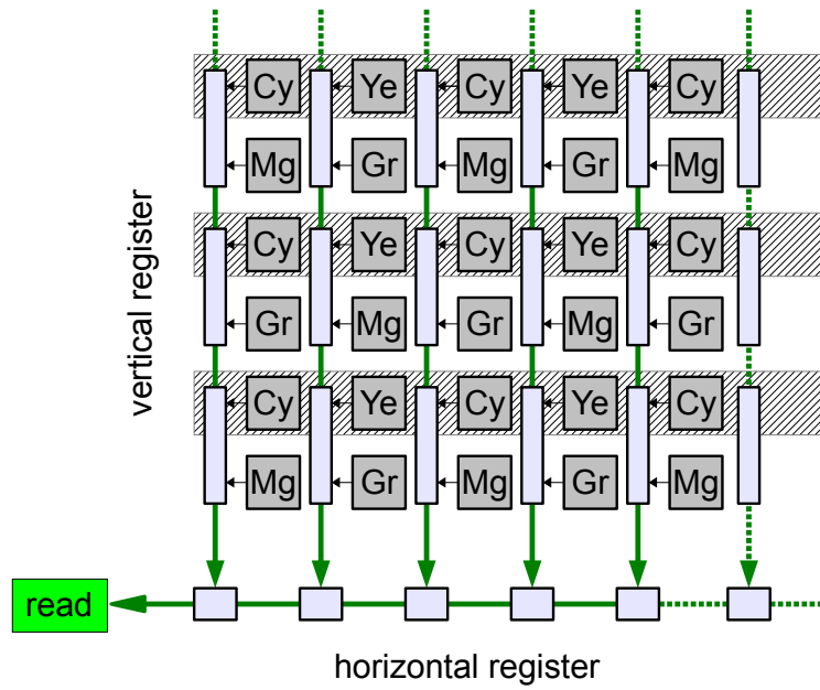
Fig. A1. Interline interlaced CMYG CCD geometry.
