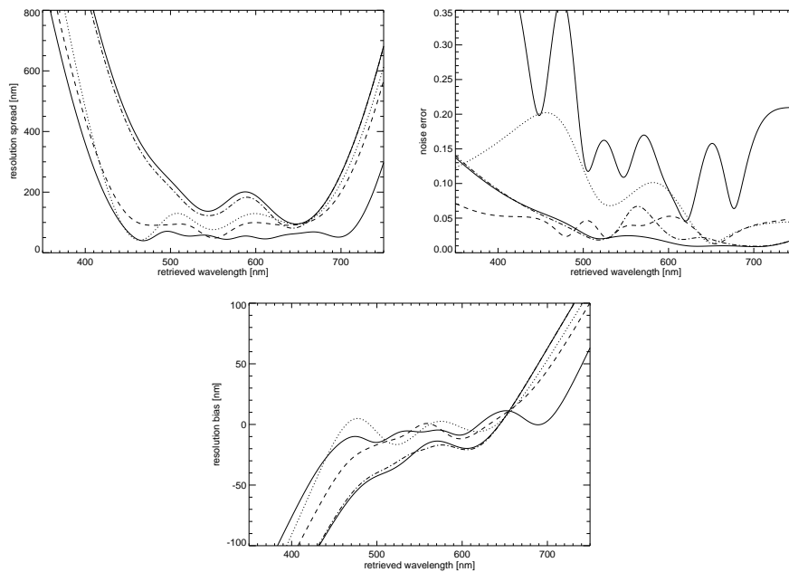
Fig. 22. Retrieval resolution ( q_2 ), noise, and bias ( q_3 ) for MX7C fast (thick solid line), MX7C raw (dotted), H9C/MX7C (dashed), 2 × MX7C with multi-notch filter (dash-dot), 3 × MX7C with two sinusoidal filters (thin solid).
