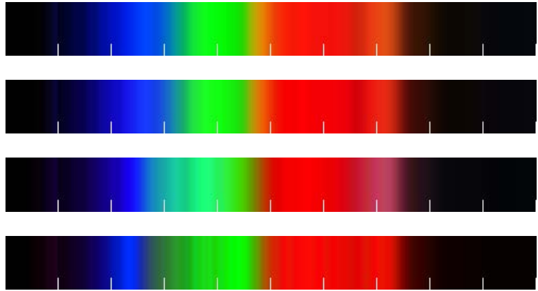
Fig. 17. Color bars for calibration wavelengths from 350 nm to 850 nm with tickmarks at 50 nm intervals. Top bar (a) is direct mapping of ICX285HQ Bayer matrix to RGB. Lower three are Backus–Gilbert estimation of CIE RGB channels for (b) ICX285HQ, (c) ICX429AKL fast mode, and (d) ICX429AKL raw mode.
